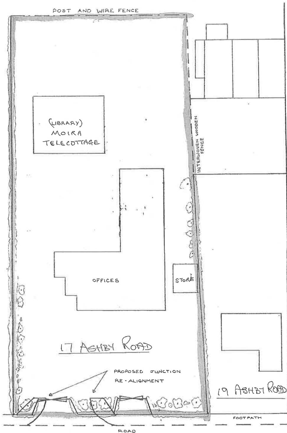
SITE PLAN
